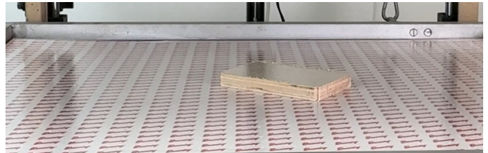
Correct package appearance with proper heating and drawdown.
